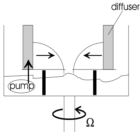
Figure 1: Sketch of radial inflow apparatus. A diffuser with a 30 cm inside diameter is constructed of wire screen (and filled with stones approximately 1cm in size), is placed in a larger tank. Water is then fed evenly in to the bottom of the diffuser. The diffuser is effective at producing an axially-symmetric, inward flow at the screen. Below the tank there is a large catch basin, partially filled with water and containing a submersible pump whose purpose is to return the water to the diffuser in the upper tank. The whole apparatus is then placed on a turntable.
