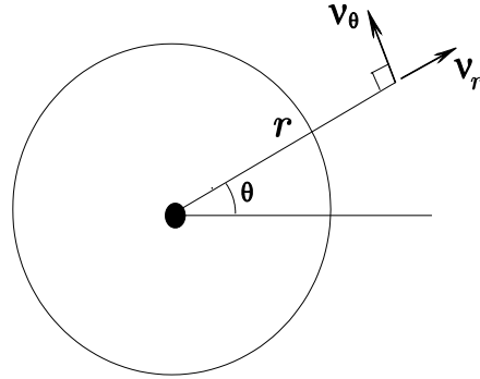
Figure 4: The velocity of a fluid parcel viewed in the rotating frame of reference: v_{rot} = (v_\theta, v_r) .
